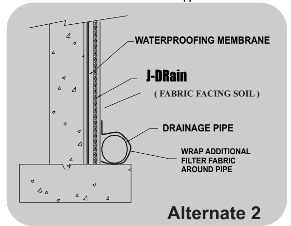
RETAINING WALL with DRAIN
