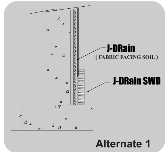
RETAINING WALL with DRAIN
